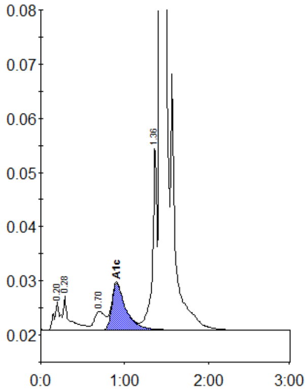
Peak table - ID: 10460790
